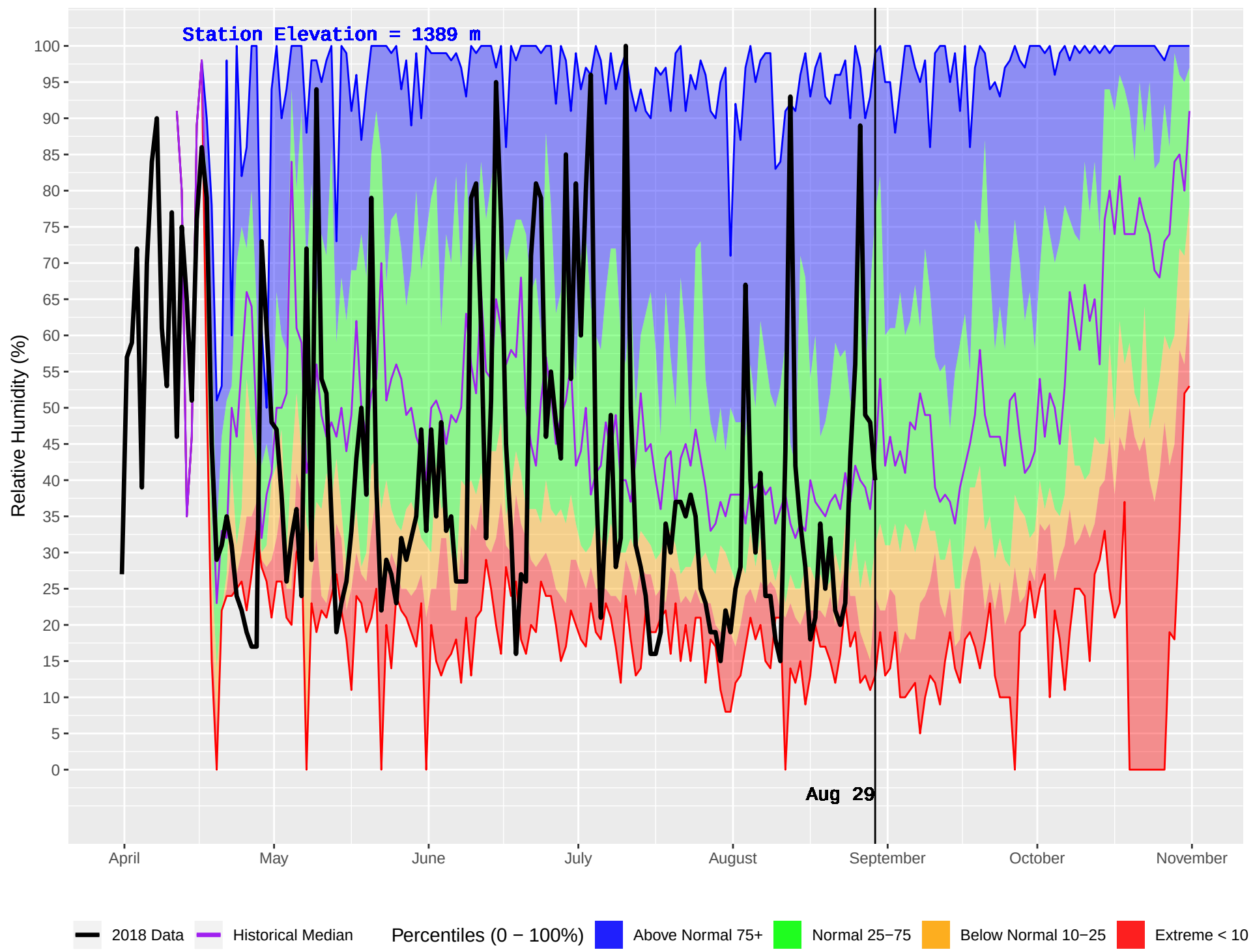
KETTLE 2 (388) : Historical (1987–2016) and Current (2018) Daily Relative Humidity
