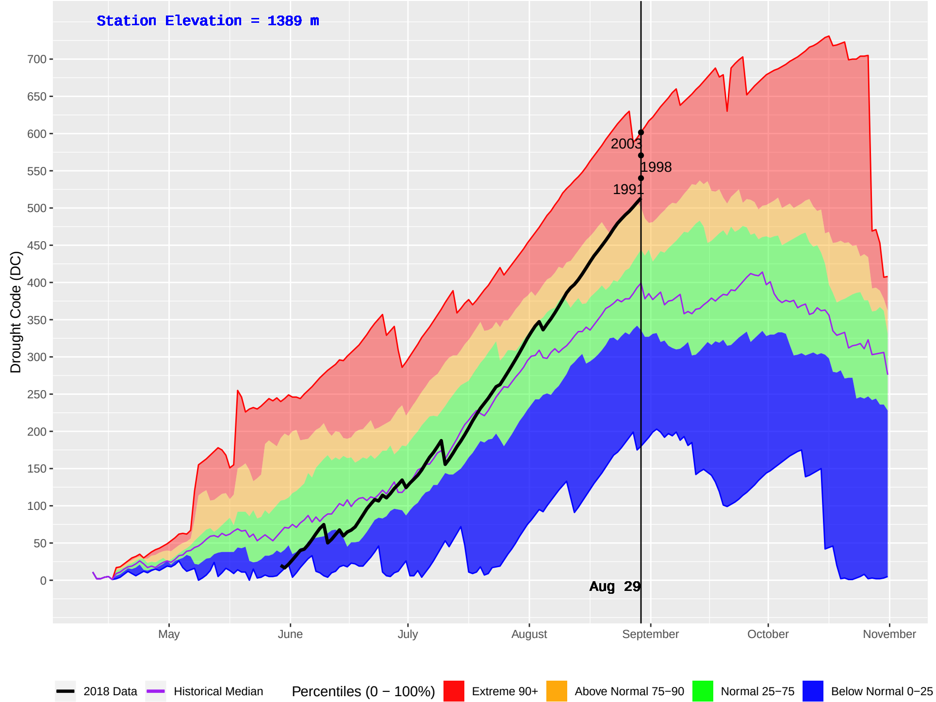
KETTLE 2 (388) : Historical (1987–2016) and Current (2018) Daily Drought Code (DC)
