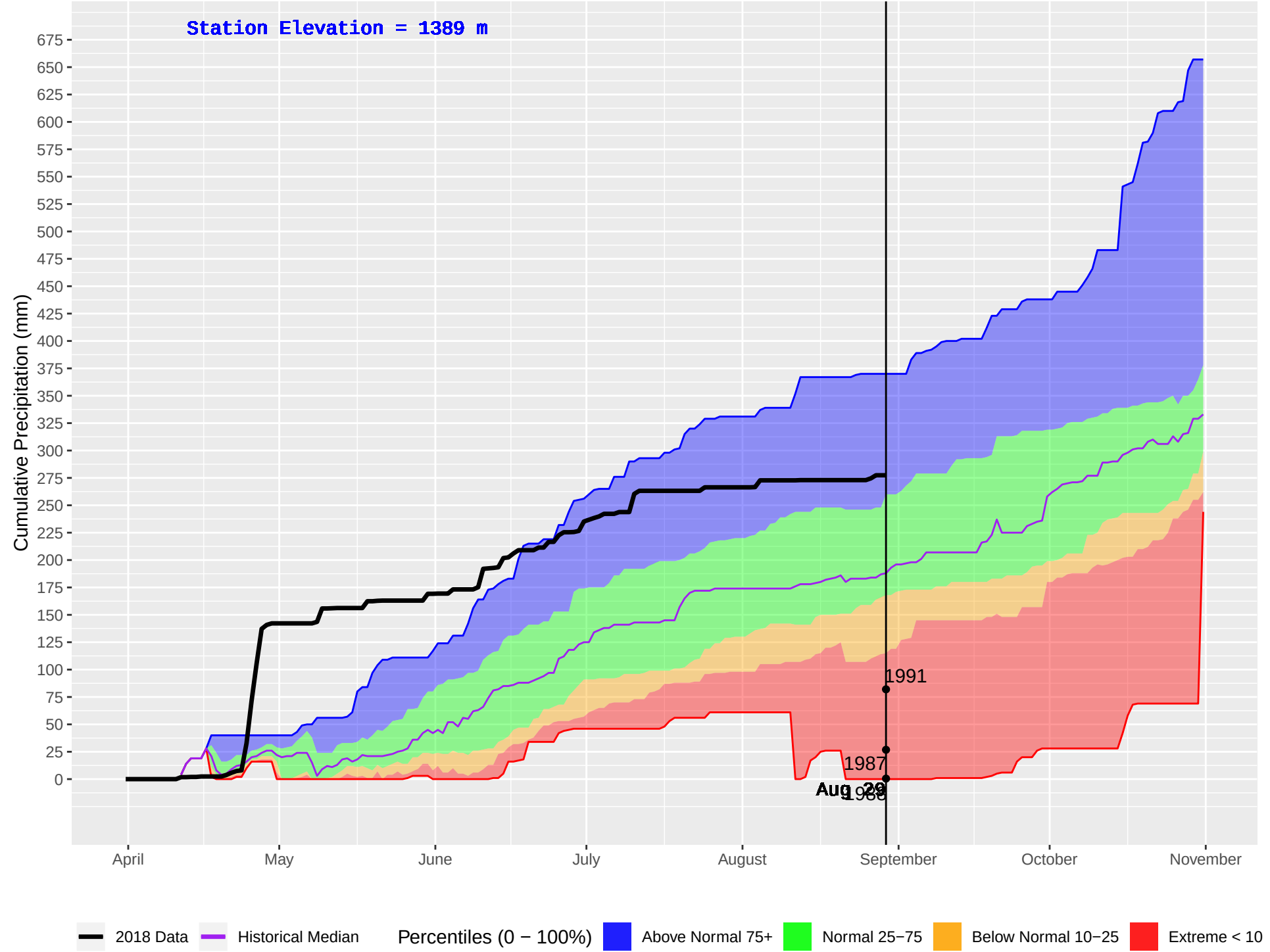
KETTLE 2 (388) : Historical (1987–2016) and Current (2018) Daily Cumulative Precipitation
