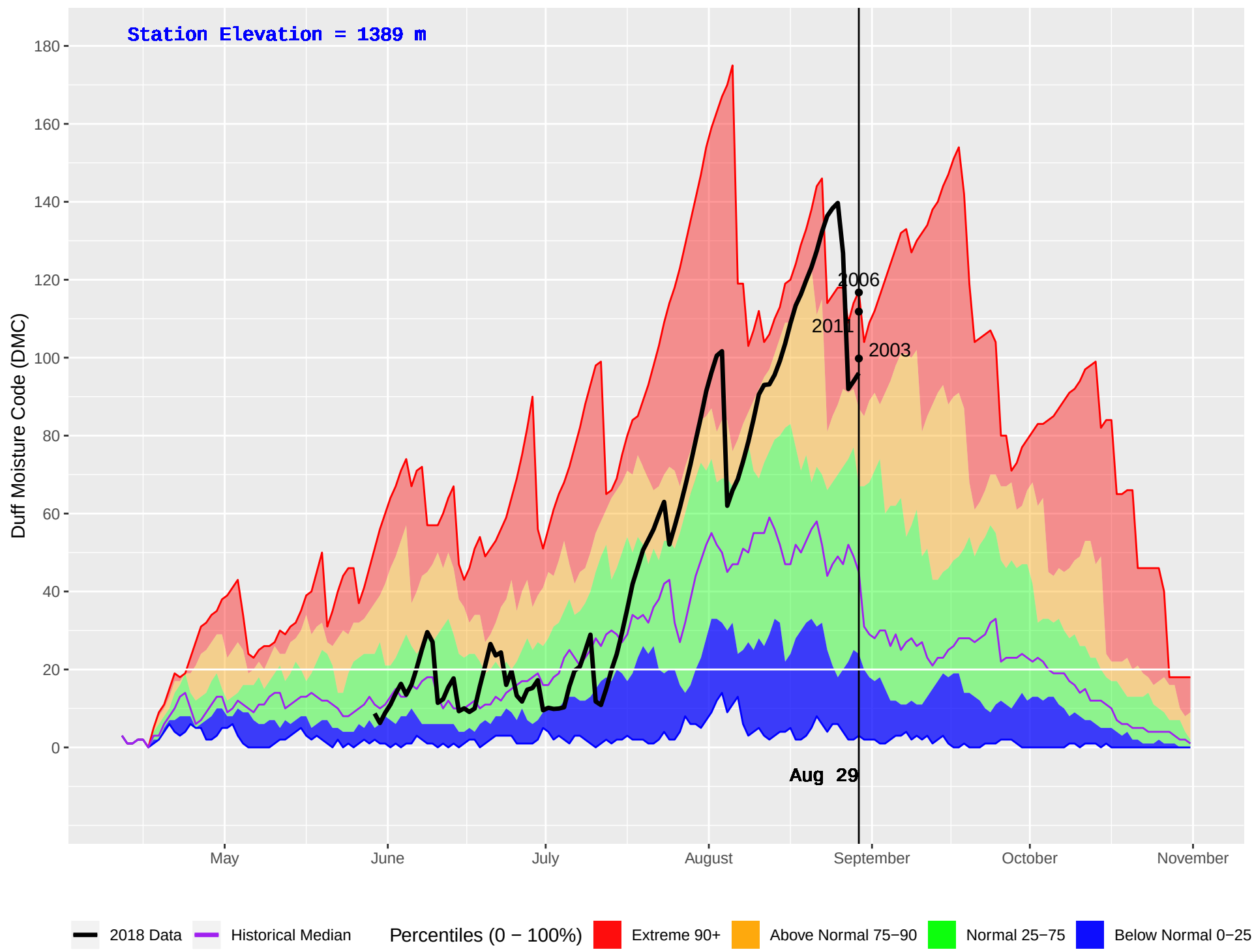
KETTLE 2 (388) : Historical (1987–2016) and Current (2018) Daily Duff Moisture Code (DMC)
