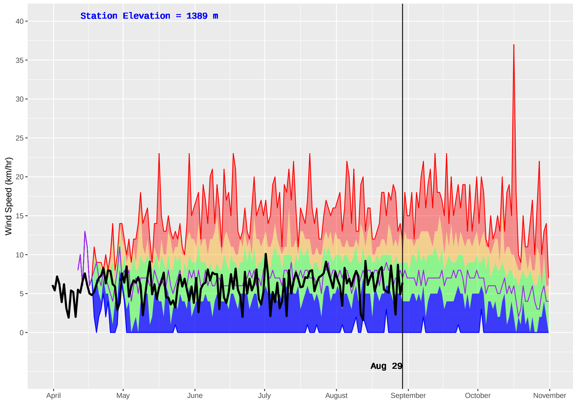
KETTLE 2 (388) : Historical (1987–2016) and Current (2018) Daily Wind Speed
