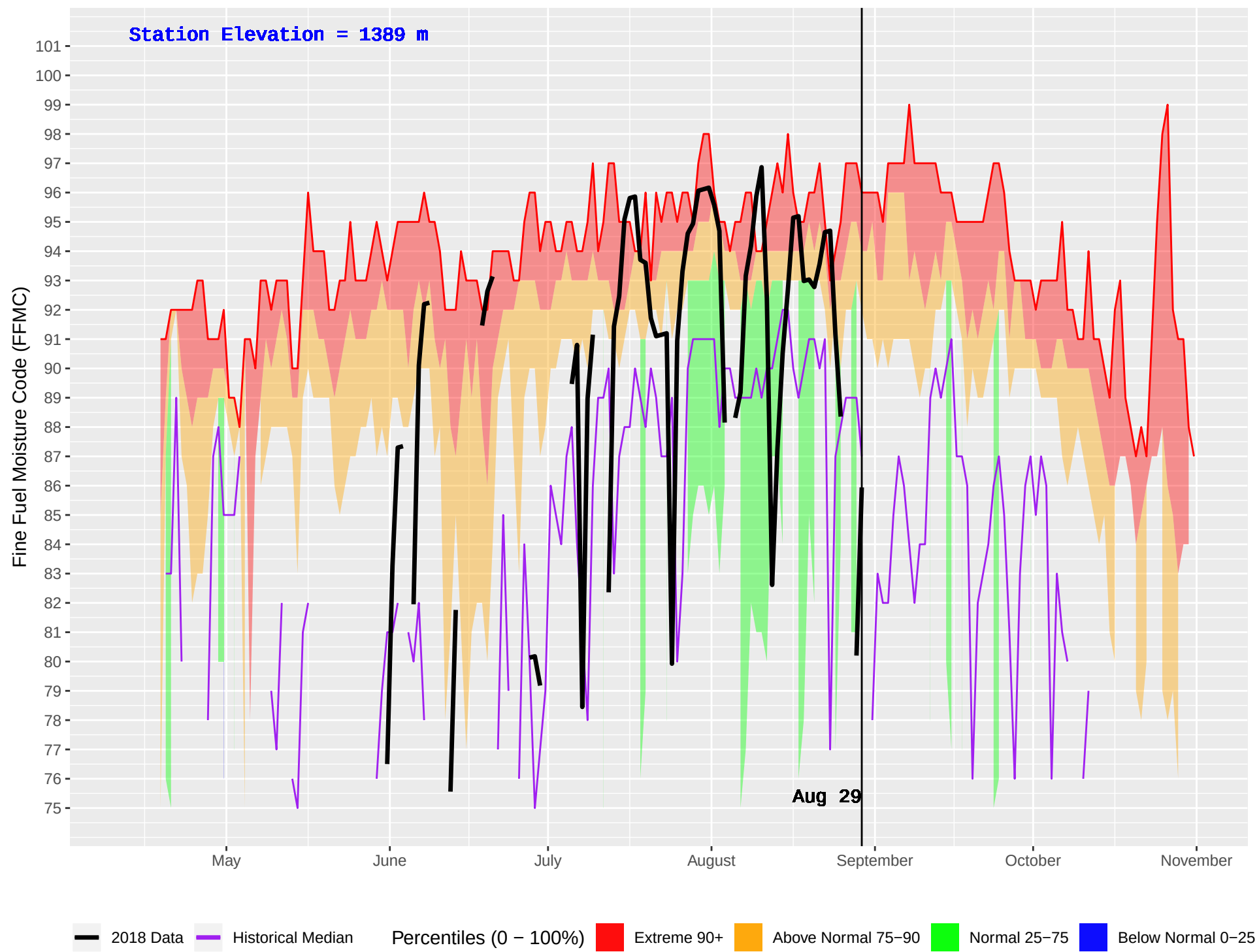
KETTLE 2 (388) : Historical (1987–2016) and Current (2018) Daily Fine Fuel Moisture Code (FFMC)
