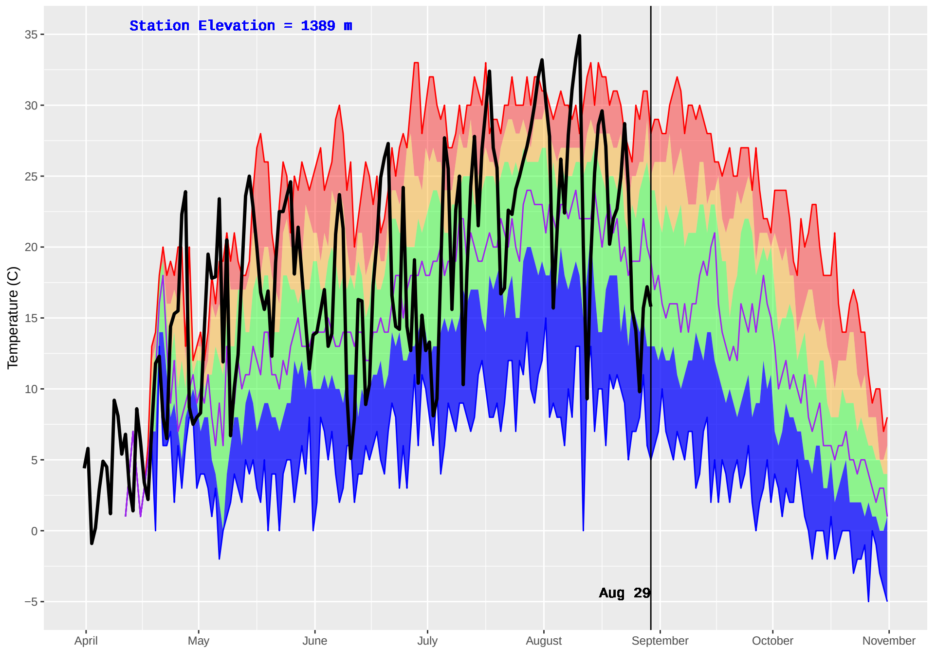
KETTLE 2 (388) : Historical (1987–2016) and Current (2018) Daily Temperature
